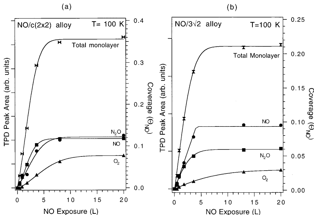
Figure 8. Uptake curves obtained from TPD results for NO adsorption kinetics at 100 K on (a) the c(2 \times 2) Sn/Pt(100) alloy and (b) the (3\sqrt{2} \times \sqrt{2})R45^\circ Sn/Pt(100) alloy.
