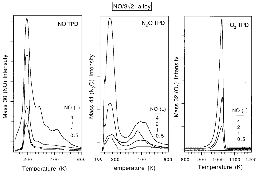
Figure 7. NO, N 2 O, and O 2 TPD traces obtained following NO exposures on the (3√2 × √2)R45°Sn/Pt(100) alloy at 100 K.
